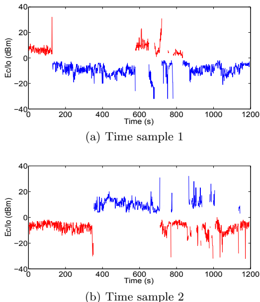
Figure 10: Typical E_c/I_o during handoffs. All E_c/I_o values are originally negative. For clarity, we flip the value to opposite, whenever a handoff happens.
