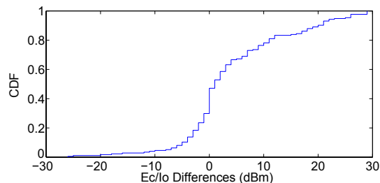
Figure 12: CDF of E_c/I_o difference between the original and new basestations during handoffs
