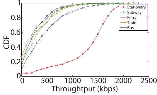
(c) Downlink of Operator B
