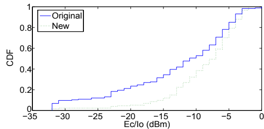
Figure 11: CDF of E_c/I_o of the original and new basestations during handoffs
