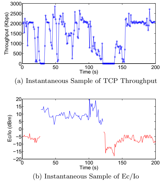
Figure 8: Impact of handoff on mobile HSDPA throughput.
