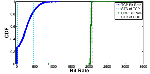
Figure 7: CDF of TCP & UDP sending bit rate in one test. TCP is more constrained and adaptive, while UDP bit rate is almost constant. STD stands for Standard Deviation.
