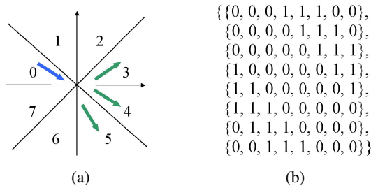
Fig. 2. An example of a partition of a view point's local tangent plane and one of the possible allowed turns encoded in matrix.
