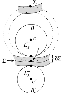
Fig. 2. A medial ball tangent to \Sigma at x (shown with dotted boundary) is shrunk radially first to the ball with dashed boundary. Then it is shrunk further to be empty of \delta\Sigma to the ball with solid boundary.
