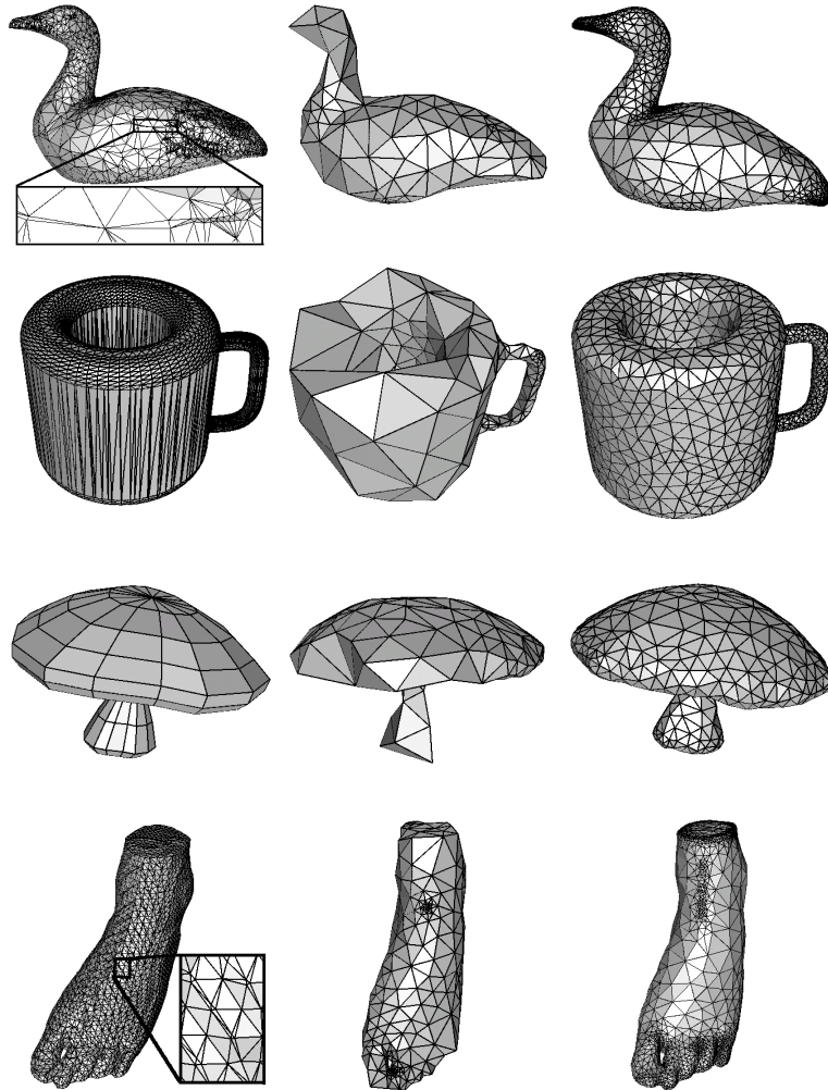
Fig. 4. The input meshes are shown in the first column. Second and third columns show the output meshes for two different levels of refinements. (a) First row shows remeshing of a reconstructed surface from a point cloud. Notice the skinny triangles present in the input. (b) Second and third rows show remeshing of a designed triangular and non-triangular surface respectively. (c) Fourth row shows remeshing of an iso-surface extracted by a marching cube algorithm from volume data. Notice that the artificial small feature created in the iso-surface is meshed densely.
