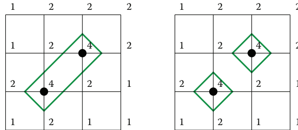
Figure 2.13. Topologically distinct isocontours created by using different isocontours for the ambiguous configuration in the central grid square.
