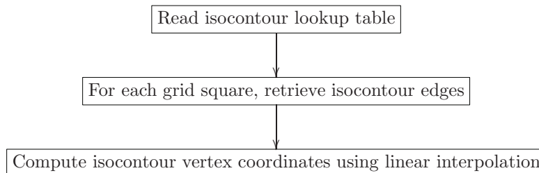
Figure 2.1. MARCHING SQUARES.
