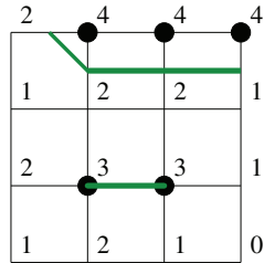
Figure 2.6. Examples of a manifold produced by MARCHING SQUARES whose boundary does not lie on the grid boundary (isovalue 3). Black vertices are positive.
