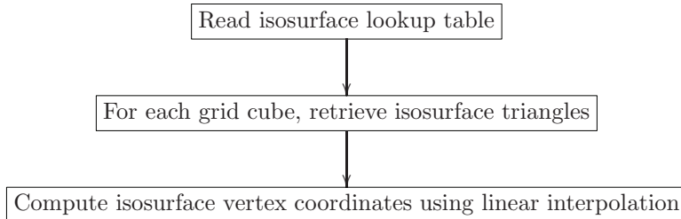
Figure 2.14. MARCHING CUBES.
