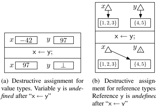
Figure 1. Leaving y undefined requires the introduction of a new value for each type: undefined. This adds additional complication to the programmer’s reasoning process; now implementers must specify and clients must understand exactly what behavior modules will have in the presence of this special value. Java programmers, especially those familiar with specifying Java in JML, know the minor mess caused by allowing null values for reference variables. The preconditions and postconditions both add extra conjuncts and implications, respectively, to ensure the desired behavior is described. The same style arises when variables are allowed to be undefined.
