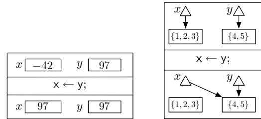
(a) Traditional preserving assignment for value types. Variable y has its original value after “ x \leftarrow y ”.
