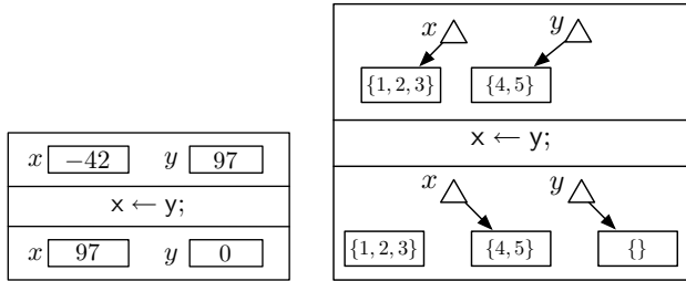
(a) Replacing assignment for value types. Variable y has some (statically) specified value after “ x \leftarrow y ”. Here 0 is given as a suitable possible value for int objects, but any set of values could be specified.
