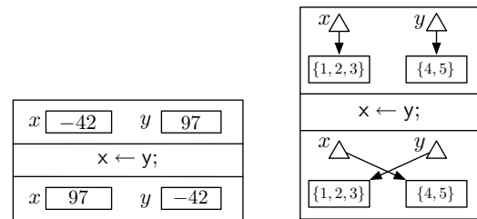
(a) Exchanging assignment for value types. Variable y has the original (old) value of x after “ x \leftarrow y ”.
