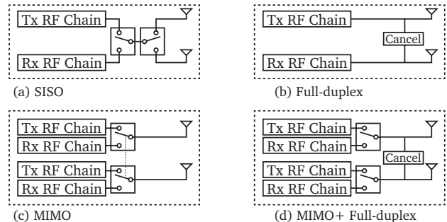
Fig. 1. Block diagram of transceiver structures with two antennas for (a) SISO half-duplex, (b) full-duplex, (c) MIMO, and (d) MIMO plus full-duplex. If a node has the transceiver structure shown in (d), then it can enable either MIMO or full-duplex communication. In transceiver structures (b) and (d), for ease of exposition, the full-duplex cancellation circuit is drawn in analogy RF end, but the cancellation can also happen in analog baseband and digital domain.
