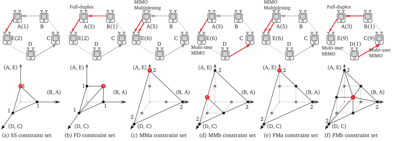
Fig. 4. Throughput regions of a five-node cyclic network under SS, FD, MMA/MMb, and FMA/FMb constraint sets. Here we only focus on the data links from A to B, from D to C and from B to A. Each dot in the throughput region plot represents a feasible schedule under the corresponding constraint set. The red arrows on each network graph illustrate one such feasible schedule, while the parentheses after each node represents its communication mode, and these feasible schedules correspond to the big red dots on the throughput region plot. (a) When every node has only one active RF chain at any time, no more than one data stream in these three links can be simultaneously activated. (b) When every node has full-duplex capability, then a data stream from B to A and a data stream from A to E can be activated together. (c,d,e) Under MMA/MMb/FMA constraint set, at any time we cannot support more than 2 simultaneous data streams in the three links. (f) When every node have both multi-user MIMO and full-duplex capabilities, three data streams, one for each data link, can be activated together. The comparison between (b,d) and (f) shows that a strictly larger throughput region can be achieved when each node can choose to operate in either MIMO or full-duplex mode, than the case when only MIMO, or only full-duplex is supported.
