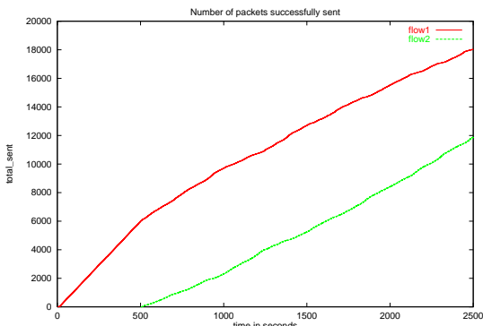
Figure 13. New Flow
