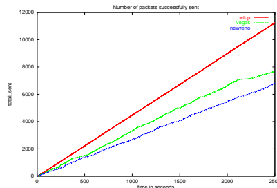
Figure 11. 6% error/20Kbps
