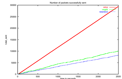
Figure 9. 6% error/50Kbps
