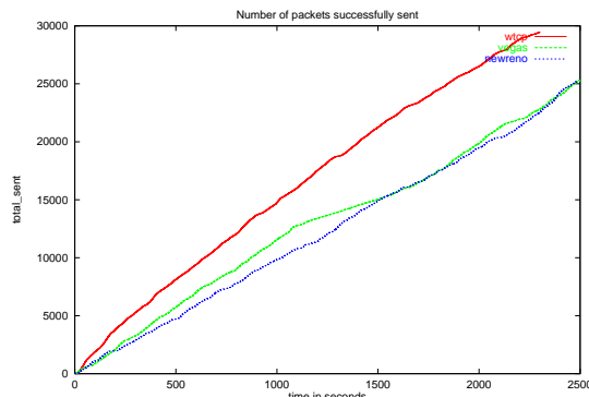
Figure 14. Aggregate sent
