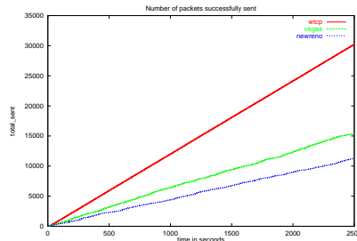
Figure 8. 4% error/50Kbps
