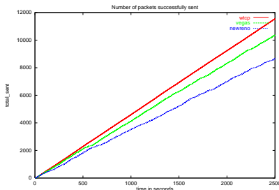
Figure 10. 4% error/20Kbps
