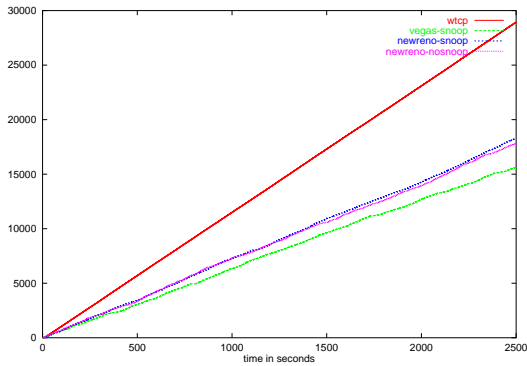
Figure 15. Snoop:50Kbps/4% error
