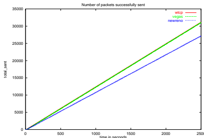
Figure 7. 0% error/50Kbps
