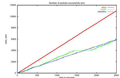
Figure 12. 8% error/20Kbps
