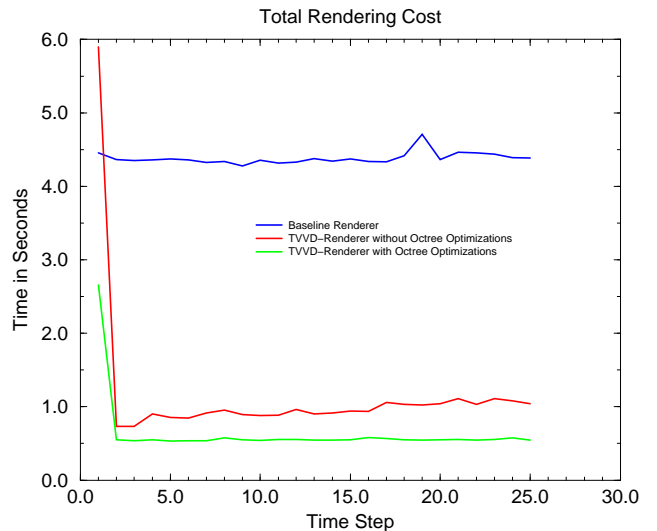
Figure 7: Rendering cost for turbulent jets dataset. The time is the total time to process, including reading encoded data from disk, unencoding when necessary, calculating gradient, rendering and compositing.
