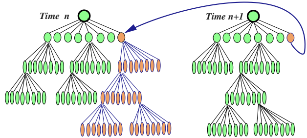
Figure 3: Merging Encoded Trees. Trees at consecutive time steps contain identical subtrees so the second time step only stores a pointer to the first time step for that subtree (red).
