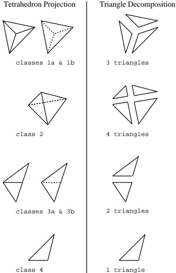
Figure 4: Decomposition of Projected Tetrahedra into Triangles
