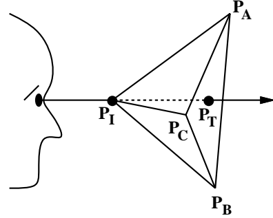
Figure 5: Example of Class 1 Decomposition.
