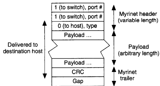
Figure 4. Myrinet packet format.
