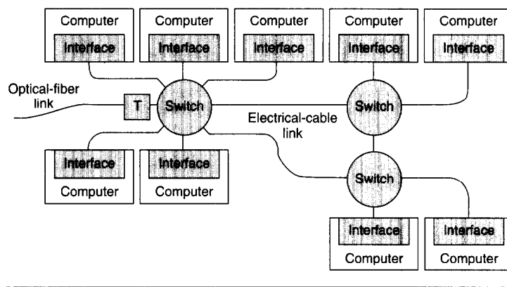
Figure 2. A possible Myrinet LAN configuration.
