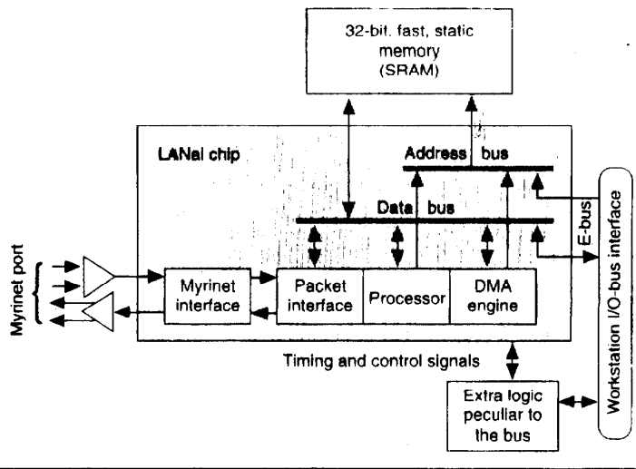
Figure 6. Host interface block diagram.
