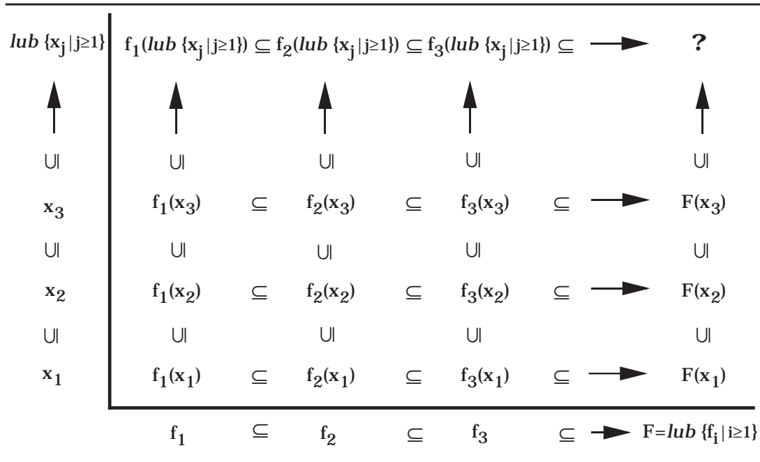
Figure 10.9: Continuity of F = \text{lub}\{f_i | i \geq 1\}
