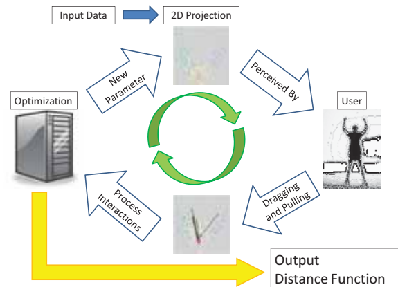
Figure 1: Flow chart showing the interactive process of using Dis-Function.
