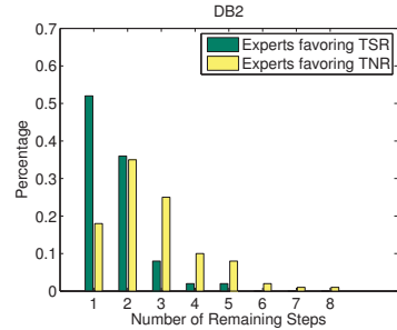
Figure 4: Efficiency of TNR vs. TSR.
