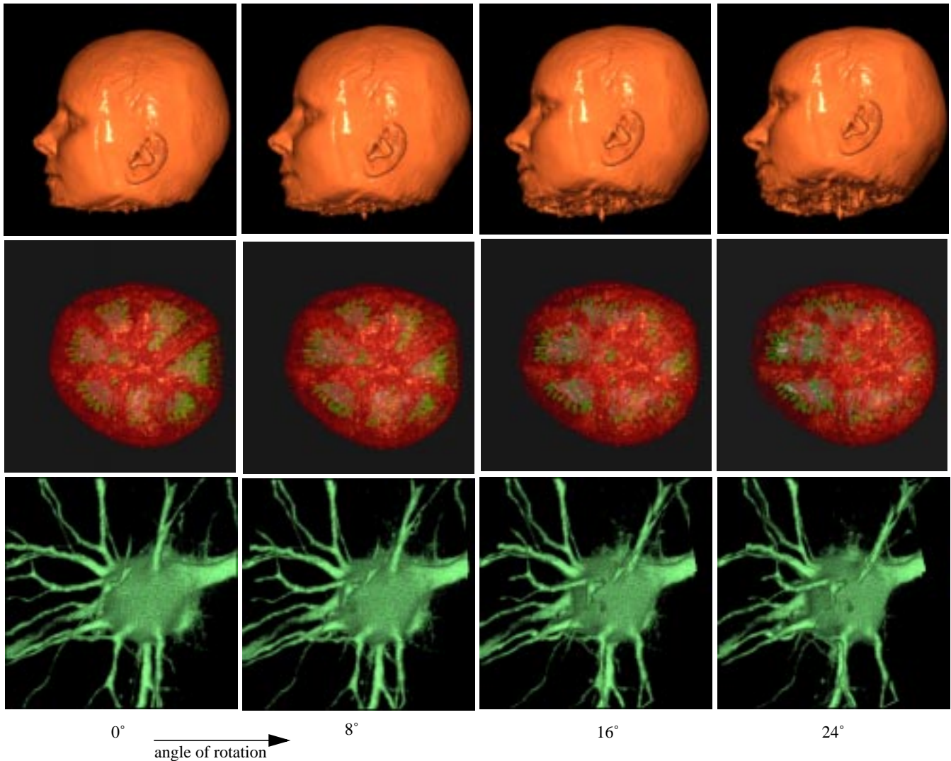
Fig. 6. IBR renderings of head, tomato and nerve datasets.
