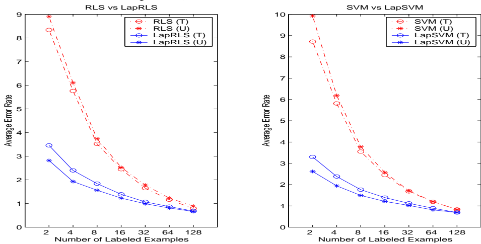
Figure 5: USPS Experiment - Mean Error Rate at Precision-Recall Break-even points as a function of number of labeled points (T: Test Set, U: Unlabeled Set)
