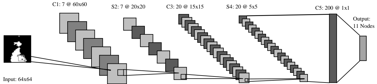
Figure 2: Architecture of a convolutional neural network for isolated digit recognition.
