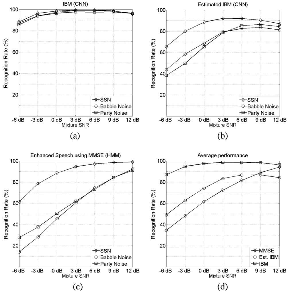
Figure 3: Recognition results using the proposed method and a traditional HMM based method. (a) Performance of the proposed method when IBMs are used. (b) Performance of the proposed method when estimated IBMs are used. (c) Performance of the HMM based speech recognizer on enhanced speech. (d) Average performance of the proposed system and the HMM based system.
