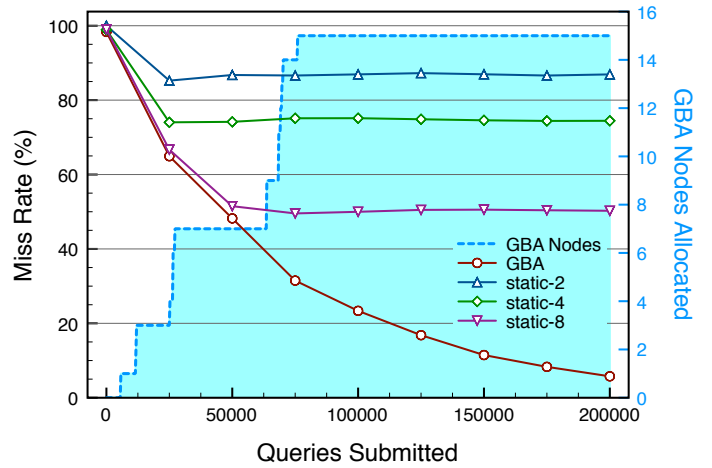
Fig. 3. Miss Rates
