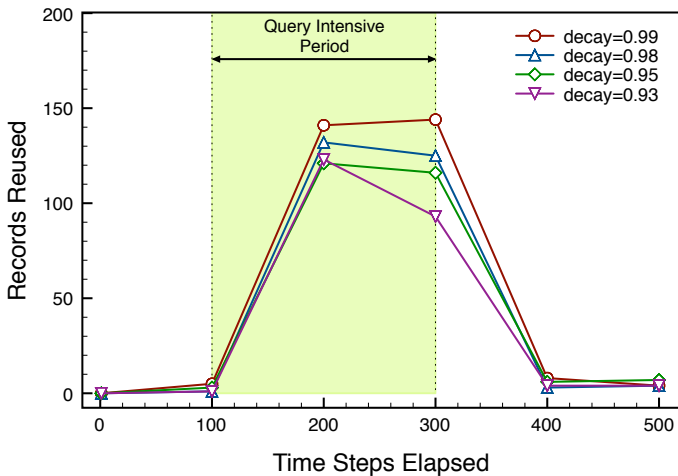
Fig. 8. Data Reuse Behavior for Various Decay \alpha = 0.99, 0.98, 0.95, 0.93
