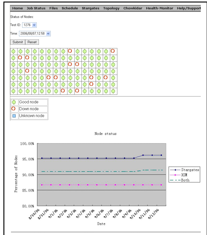
Fig. 2. Visualization of Kansei health using Chowkidar.
