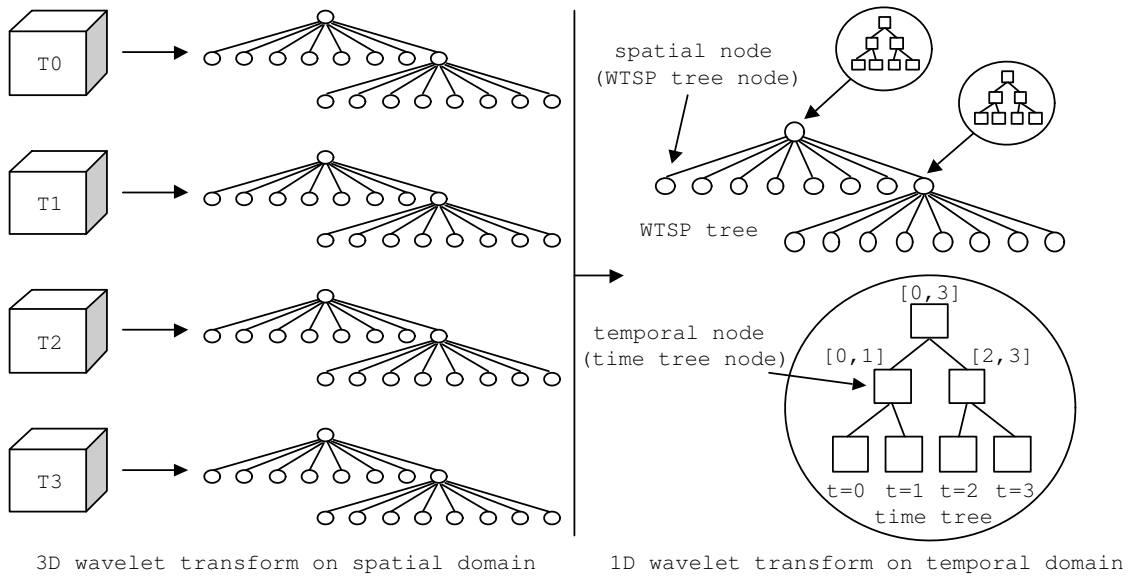
Figure 2: The conceptual diagram of performing a two-stage wavelet transform process on time-varying volume data in spatial and temporal domains using WTSP tree. The volume at each time step is subdivided into a sequence of blocks, which correspond to the leaf nodes of the WTSP tree. For each spatial node in the WTSP tree, a 3D wavelet transform is performed on its data block, resulting in low-pass and high-pass filtered coefficients. Then, low-pass filtered coefficients are gathered by its parent node to build up the spatial hierarchy recursively while high-pass filtered coefficients across all the time steps undergo 1D wavelet transforms to build up the temporal wavelet hierarchy at that node. In this example, the time-varying data has four time steps.
