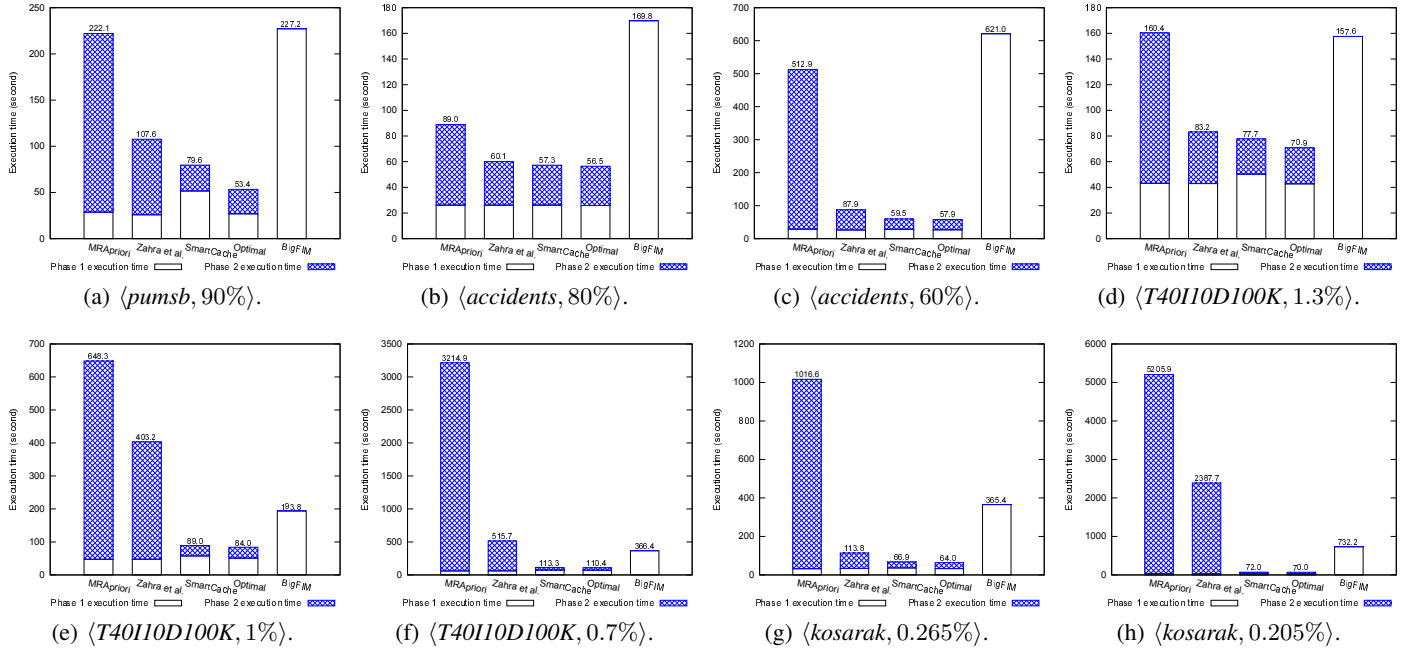
Fig. 10: Execution time comparison for different datasets and minimum support values.
