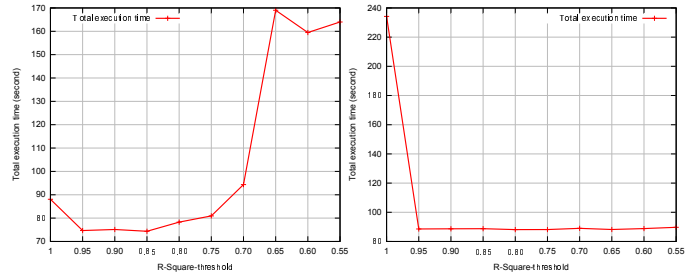
(a) \langle pumsb, 90\% \rangle .
