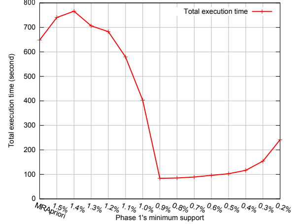
Fig. 9: Execution time as a function of phase 1's minimum support. Inputs are \langle T40I10D100K, 1\% \rangle .
