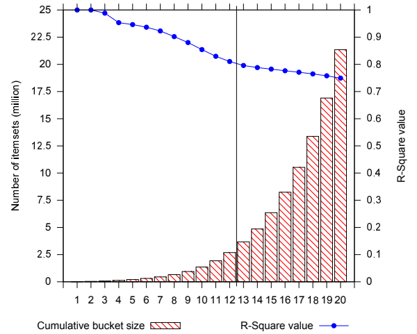
Fig. 6: SmartCache online analyzer’s working logic in detail. It shows the cumulative bucket size trend, and the R-Square value trend. The statistics are from one Map task in phase 1. Inputs are \langle pumsb, 85\% \rangle .
