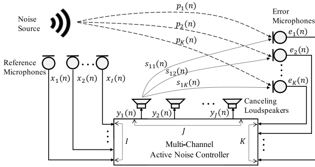
Fig. 1. Diagram of a general I \times J \times K multi-channel active noise control system that consists of I reference microphones, J canceling loudspeakers, and K error microphones. Symbol p_k denotes the primary path from the noise source to the k th error microphone, and s_{jk} denotes the secondary path from the j th canceling loudspeaker to the k th error microphone.
