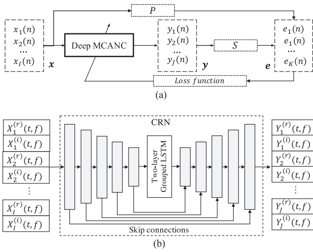
Fig. 2. Diagram of (a) deep MCANC approach, and (b) CRN based deep MCANC. P and S denoted primary and secondary paths. Superscripts (r) and (i) denote real and imaginary parts of signals, respectively.
