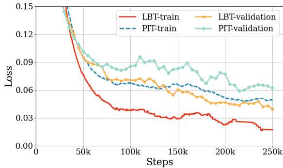
Fig. 3. Comparison of diarization loss curves ( L_{\text{END}} ) in training and validation with LBT and PIT criteria.
