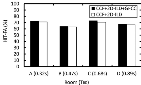
Fig. 9. Two-source segregation with binaural-only and binaural-monaural features in four reverberant rooms at the input SNR of 0 dB.
