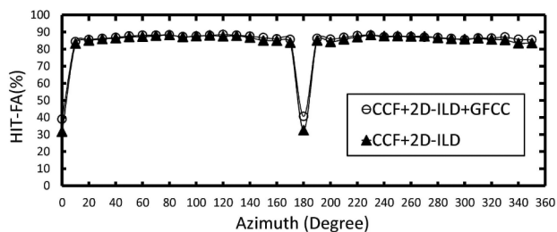
Fig. 6. HIT-FA performance for two-source segregation on the 0-dB test set.
