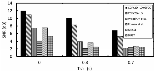
Fig. 8. SNR comparisons in the 5-source environment where speech utterances are mixed with the babble noise at 0 dB.
