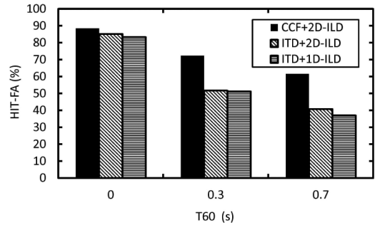
Fig. 2. Two-source segregation for trained azimuths at 0-dB SNR.
