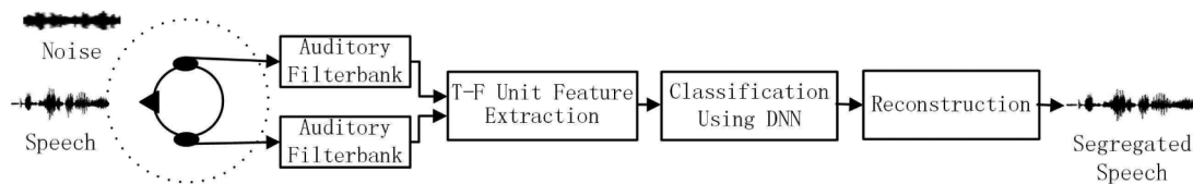
Fig. 1. Schematic diagram of the proposed binaural DNN classification system.
