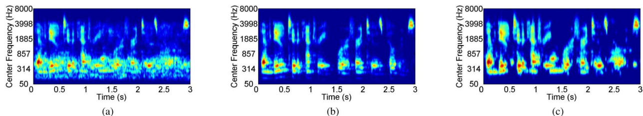
Fig. 10. Segregation illustration for a TIMIT utterance mixed with babble noise in Room C at 0-dB SNR. (a) Cochleagram of the reverberant mixture. (b) Cochleagram of the reverberant target utterance. (c) Cochleagram of separated speech.
