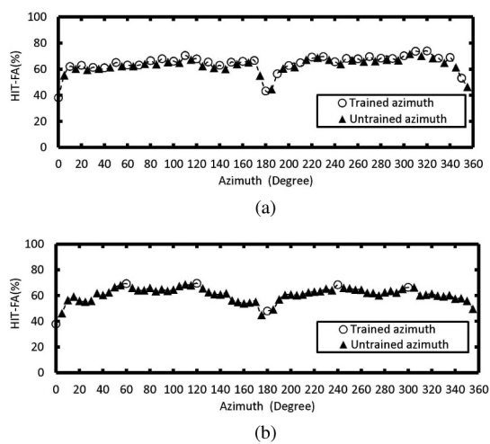
Fig. 7. HIT-FA performance for two-source segregation at various interference training azimuths with joint features in the reverberant condition at 0 dB. (a) 36 interference azimuths are used in training. (b) 6 interference azimuths are used in training.
